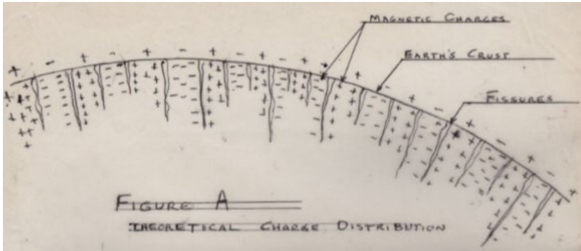
Figure A shows the theory that the earth is a huge dynamo spinning in space, charged alternately positive and negative, this in turn would generate magnetic lines of force. These lines would tend to draw the rods parallel to the direction of the fault when stepping from one charge to the opposite charge.
